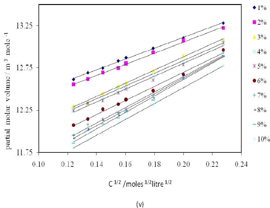
Fig. 1. Variation of partial molar volumes, V_{\phi} vs. molar concentration, C of l - leucine in ethanol + water (w/w) solutions, at (i) 298.15 K, (ii) 303.15 K, (iii) 308.15 K, (iv) 310.15 K, (v) 313.15 K,
