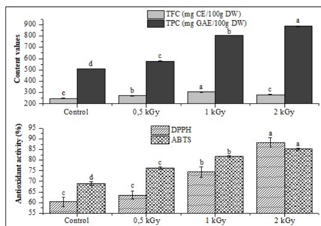
Figure 1: Total phenolics content, total flavonoids content and antioxidant activity of irradiated samples compared to the control (unirradiated sample).
