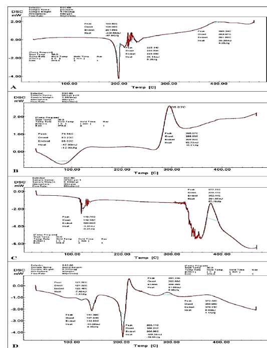
Figure 1. DSC curves A: pure piroxicam, B: pure chitosan, C: pure HPMC, D: F5 formulation.
