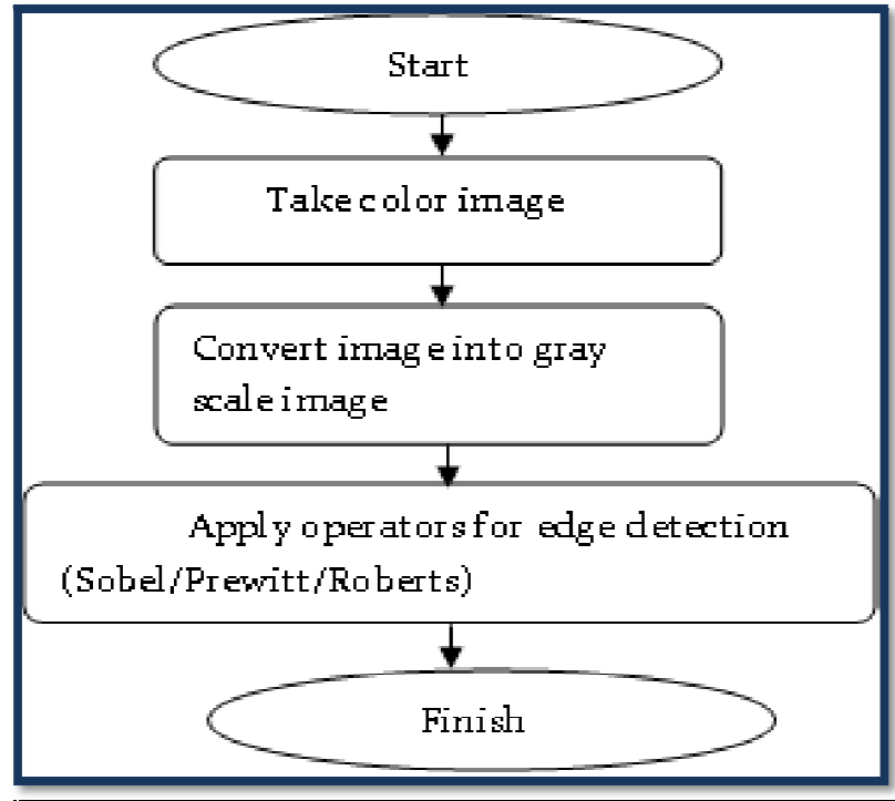
Fig 3. General process of edge detection 36
