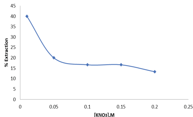
Figure 4 Effect of salt on cobalt extraction.
