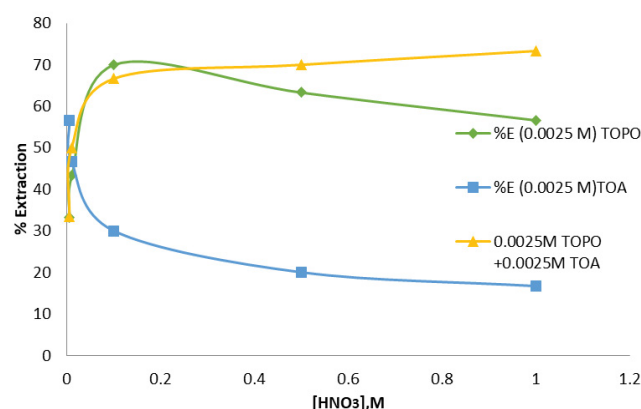
Figure 1 Effect of nitric acid concentration on cobalt extraction.
