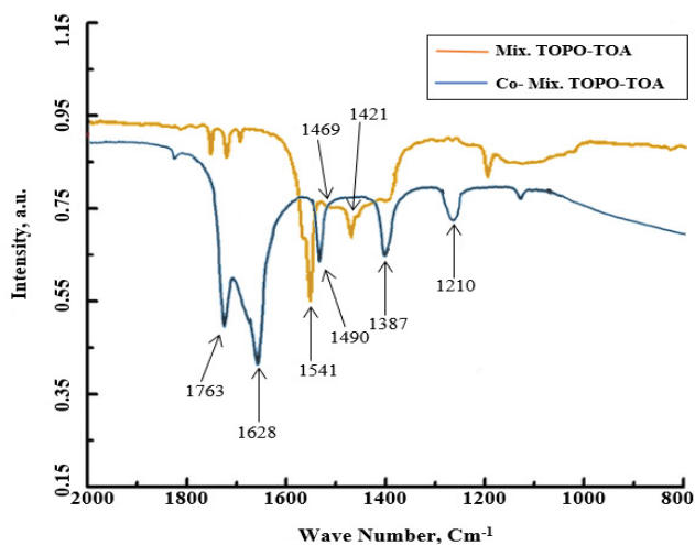
Figure 5 FTIR spectra of mixture of TOPO and TOA in cyclohexane and cobalt loaded mixture of TOPO and TOA in cyclohexane.
