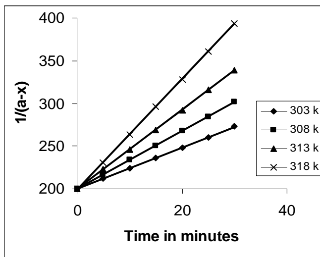
Fig:2 Plot of 1/(a-x) versus t
