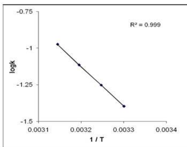
Fig.3 Plot of \log k versus 1/T
