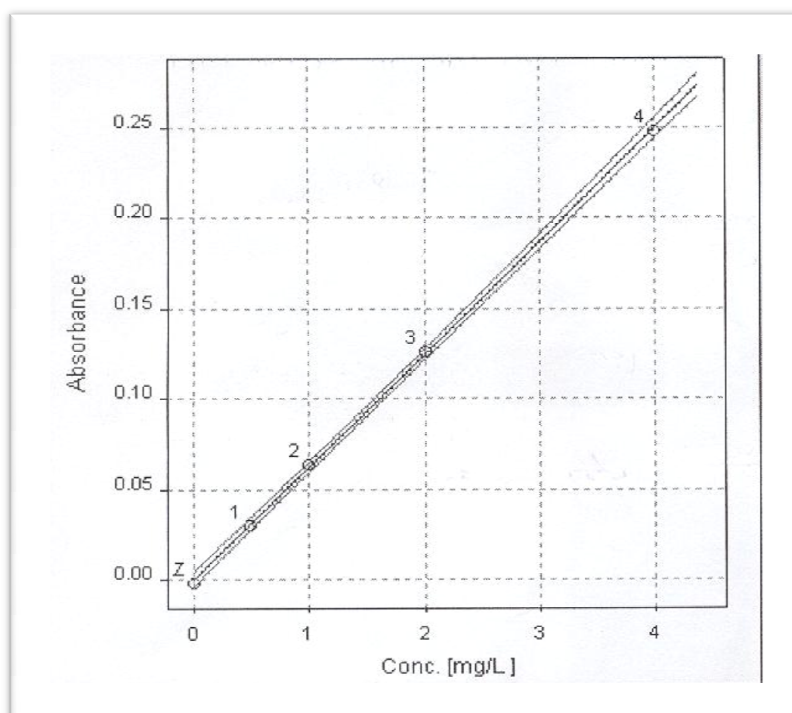
Figure (1): The calibration curve of Cu 2+ by FAAS.
