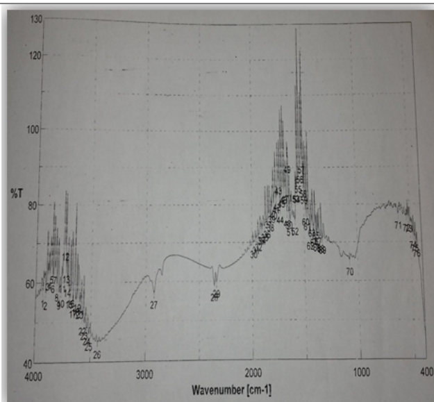
Figure 2: ATR-FTIR analysis of ( Penicillium italicum SSF extract).
